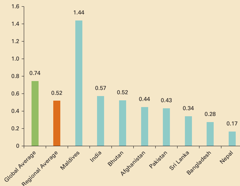
Figure 3.26 Waste Generation Rates: South Asia Region kg/capita/day
