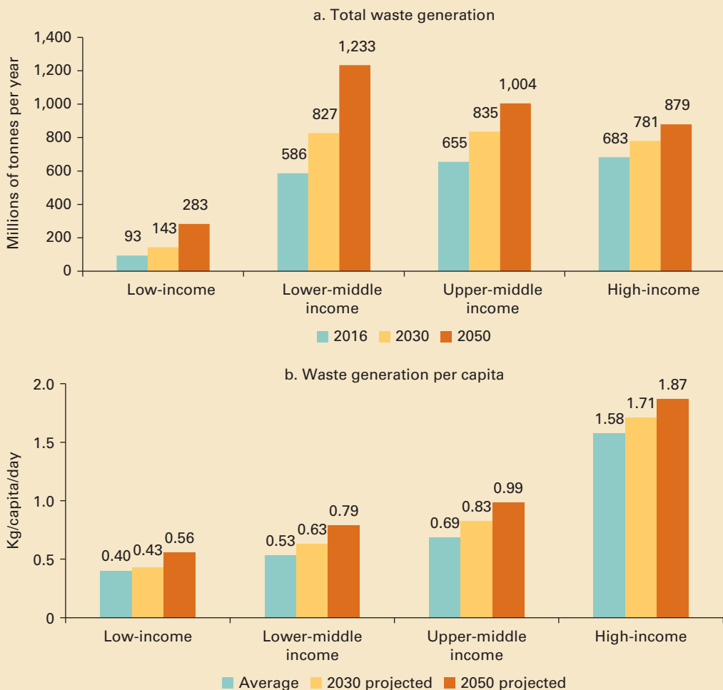
Figure 2.6 Projected Waste Generation by Income Group
