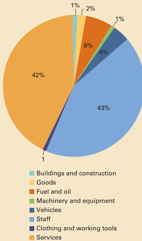
Figure 7.2.3 Urban Solid Waste Management by Spending Category in Argentina
